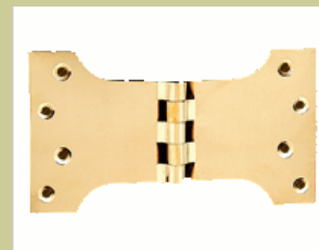
MJK AI PH Solid Brass Parliament Hinges With Stainless Steel Fitting Pin Size : 75 x 50 mm (3' x 2") 75 x 75 mm (3' x 3") 100 x 50 mm (4' x 2") 100 x 75 mm (4' x 3") 100 x 100 mm (4' x 4") 100 x 125 mm (4' x 5") 100 x 150 mm (4' x 6") 125 x 125 mm (5' x 5") 125 x 150 mm (5' x 6")
